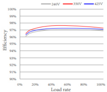
Efficiency curve
